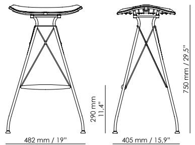
OD15-75 Suitable for bar height
